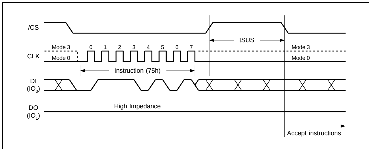
Figure 29a. Erase/Program Suspend Instruction (SPI Mode)
