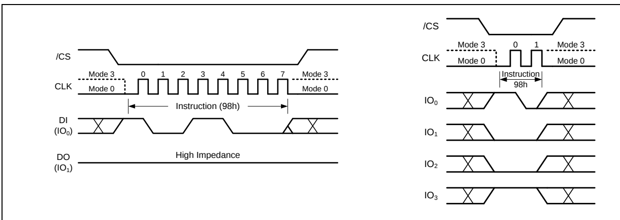
Figure 51. Global Block Unlock Instruction for SPI Mode (left) or QPI Mode (right)
