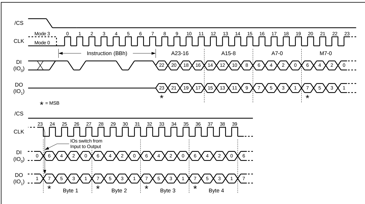
Figure 17a. Fast Read Dual I/O Instruction (Initial instruction or previous M5-4 ≠ 10, SPI Mode only)
