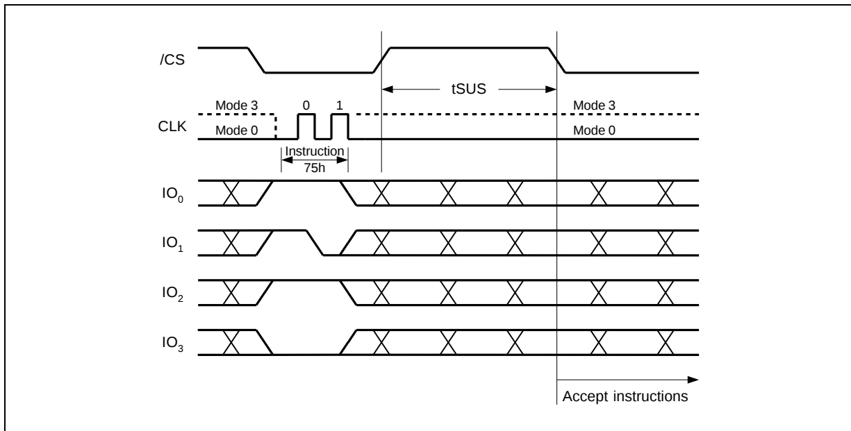
Figure 29b. Erase/Program Suspend Instruction (QPI Mode)
