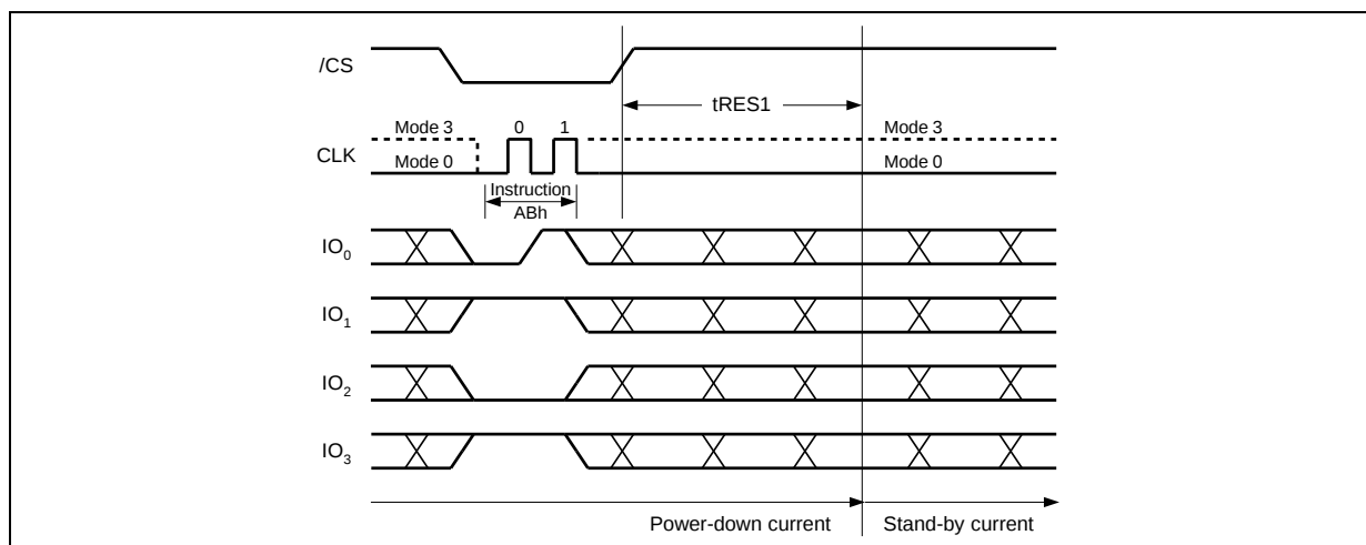
Figure 32b. Release Power-down Instruction (QPI Mode)
