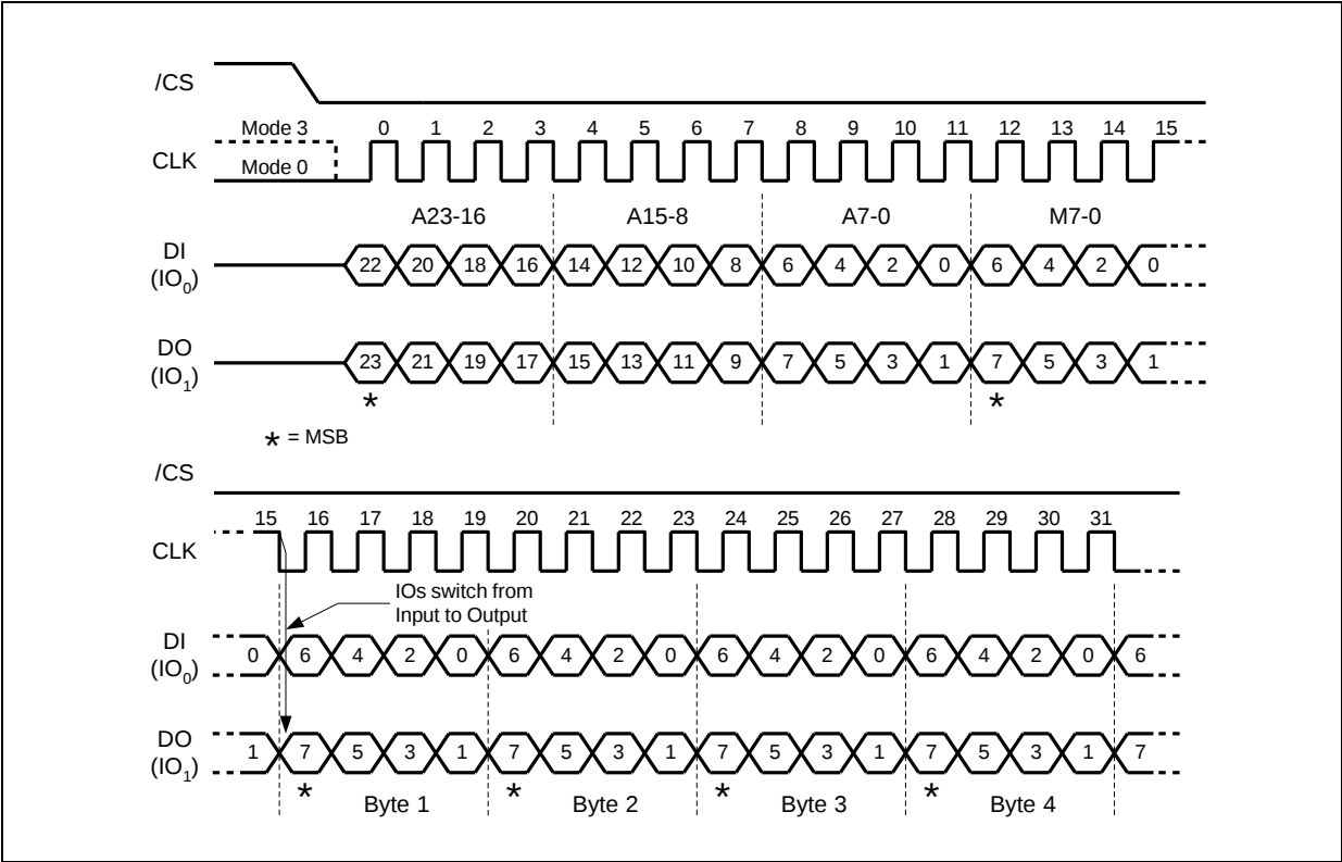
Figure 17b. Fast Read Dual I/O Instruction (Previous instruction set M5-4 = 10, SPI Mode only)
