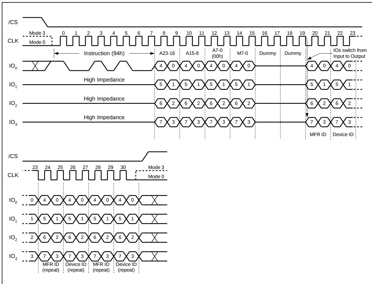
Figure 35. Read Manufacturer / Device ID Quad I/O Instruction (SPI Mode only)
