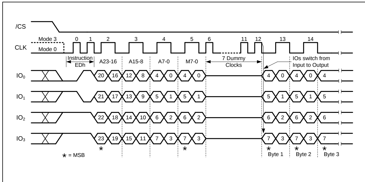
Figure 21a. DTR Fast Read Quad I/O (Initial instruction or previous M5-4≠10, QPI Mode)
