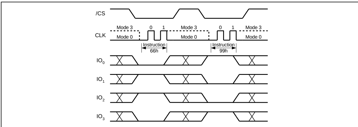
Figure 52b. Enable Reset and Reset Instruction Sequence (QPI Mode)
