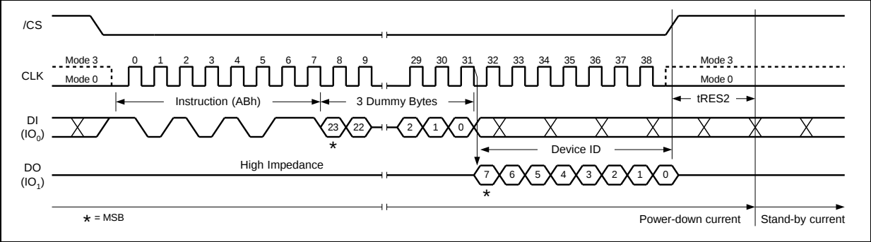
Figure 32c. Release Power-down / Device ID Instruction (SPI Mode)
