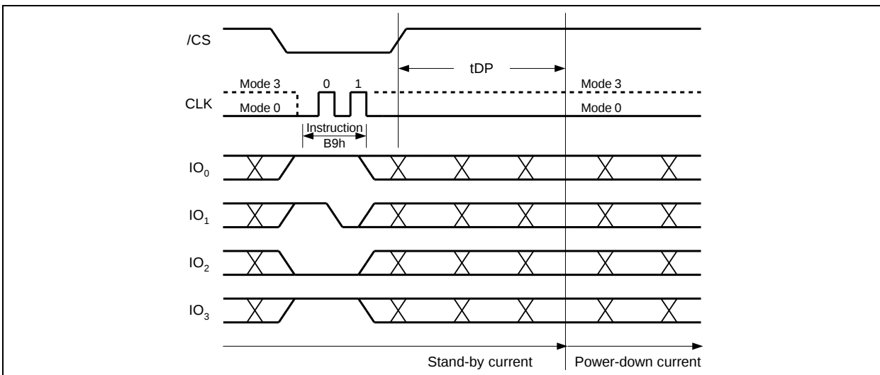
Figure 31b. Deep Power-down Instruction (QPI Mode)
