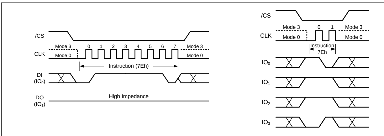
Figure 50. Global Block Lock Instruction for SPI Mode (left) or QPI Mode (right)
