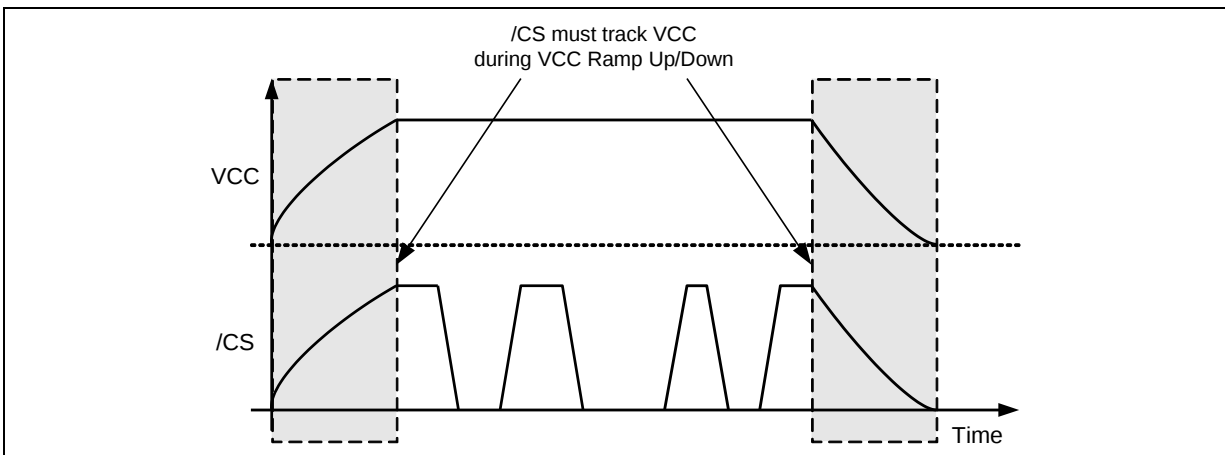
Figure 53b. Power-up, Power-Down Requirement
