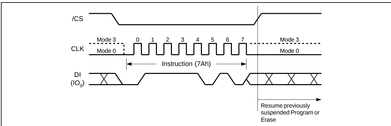
Figure 30a. Erase/Program Resume Instruction (SPI Mode)
