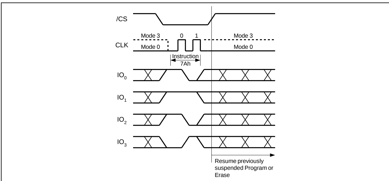
Figure 30b. Erase/Program Resume Instruction (QPI Mode)
