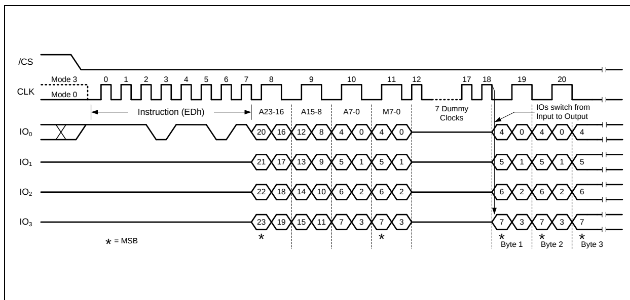
Figure 20a. DTR Fast Read Quad I/O (Initial instruction or previous M5-4≠10, SPI Mode)
