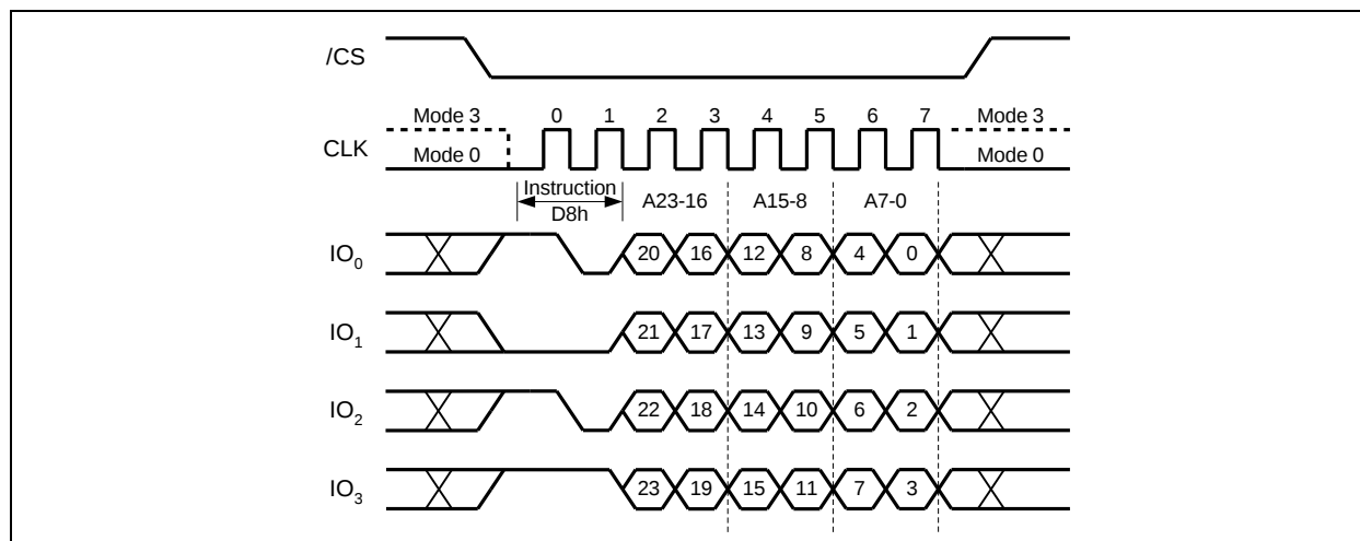
Figure 27b. 64KB Block Erase Instruction (QPI Mode)
