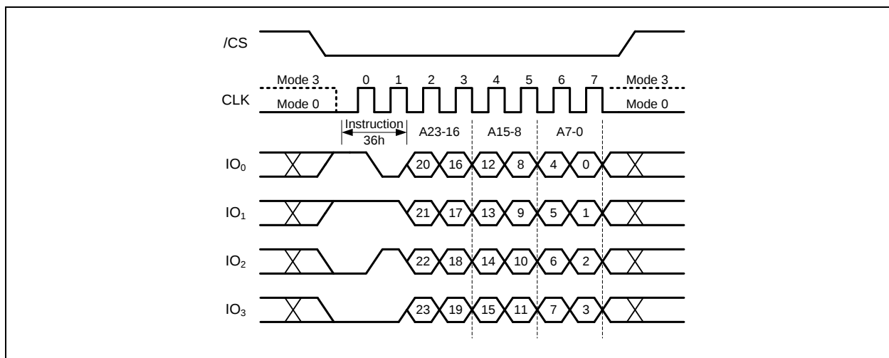
Figure 47b. Individual Block/Sector Lock Instruction (QPI Mode)
