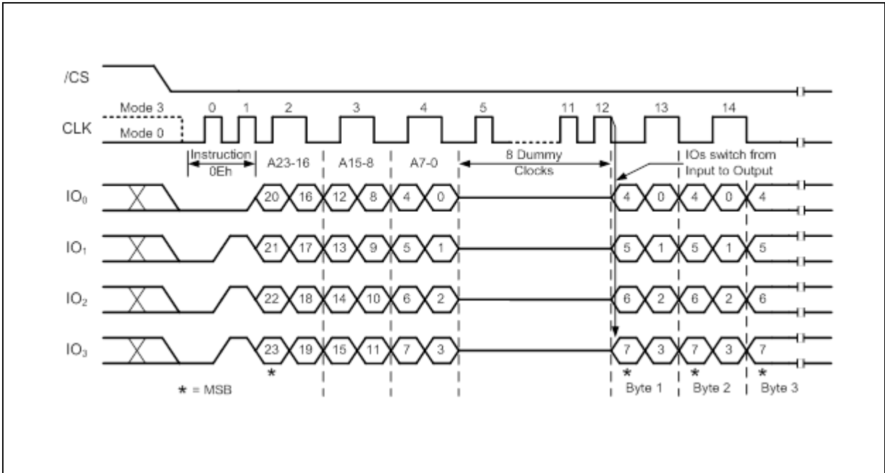
Figure 44. DTR Burst Read with Wrap Instruction (QPI Mode only)
