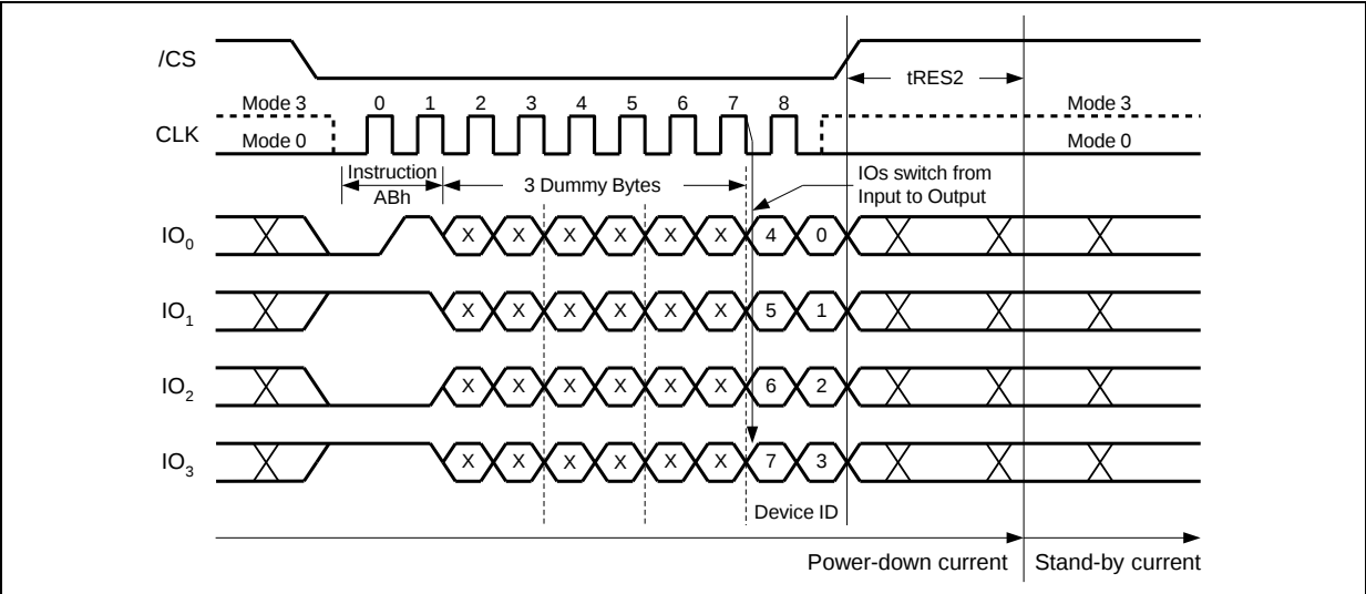
Figure 32d. Release Power-down / Device ID Instruction (QPI Mode)
