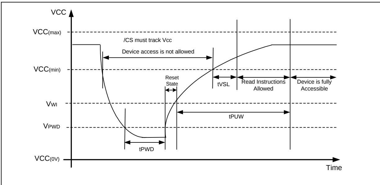
Figure 53a. Power-up Timing and Voltage Levels
