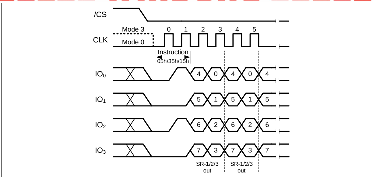
Figure 9b. Read Status Register Instruction (QPI Mode)
