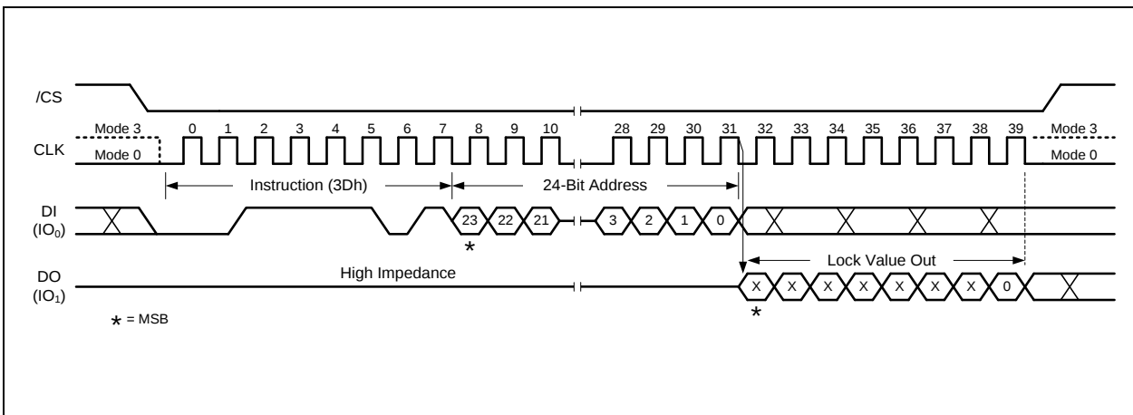
Figure 49a. Read Block Lock Instruction (SPI Mode)
