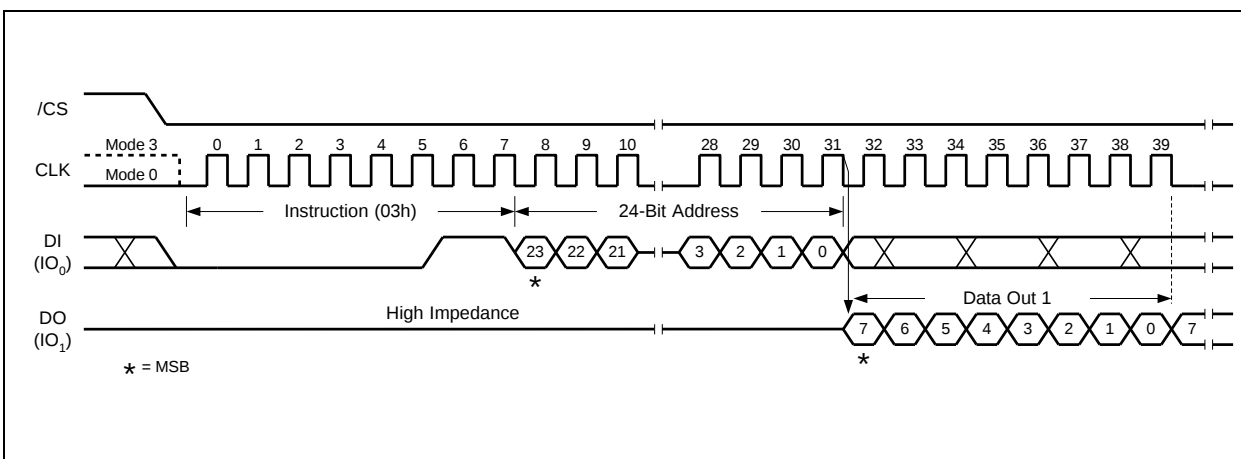
Figure 12. Read Data Instruction (SPI Mode only)
