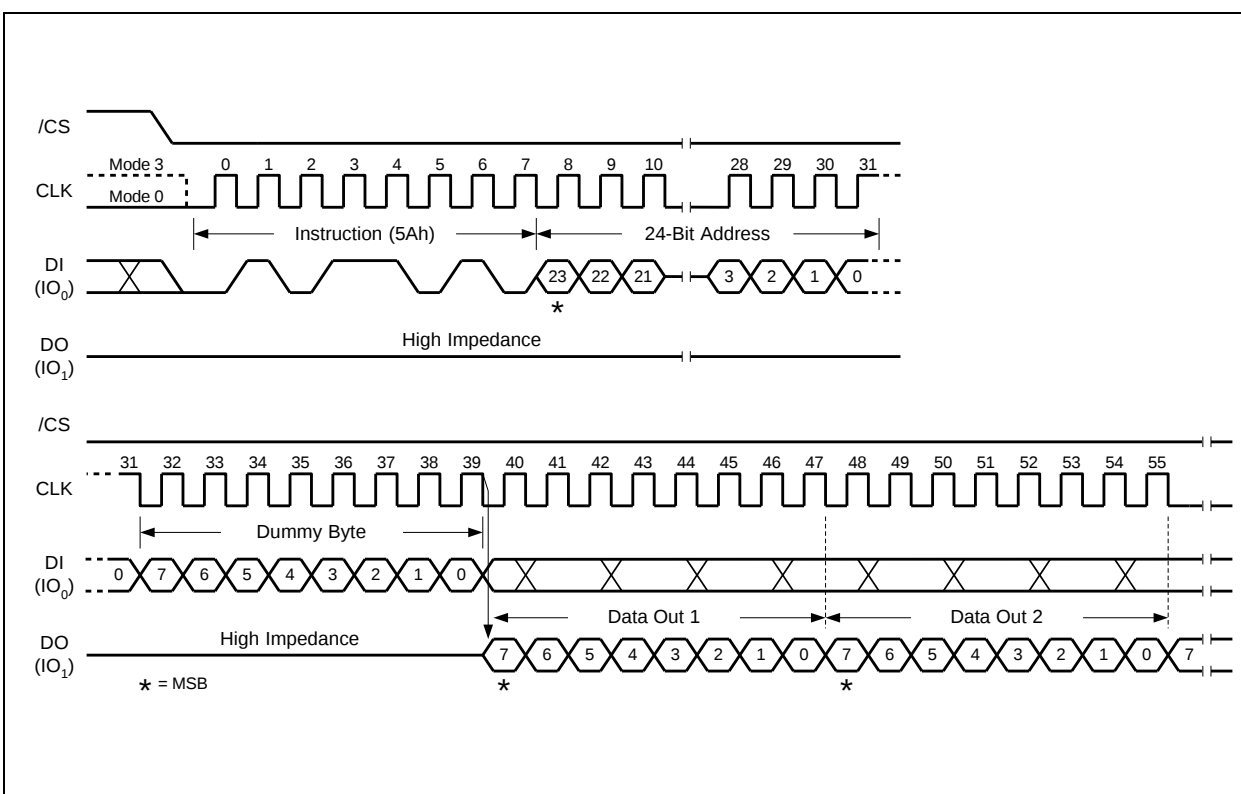
Figure 38. Read SFDP Register Instruction Sequence Diagram
