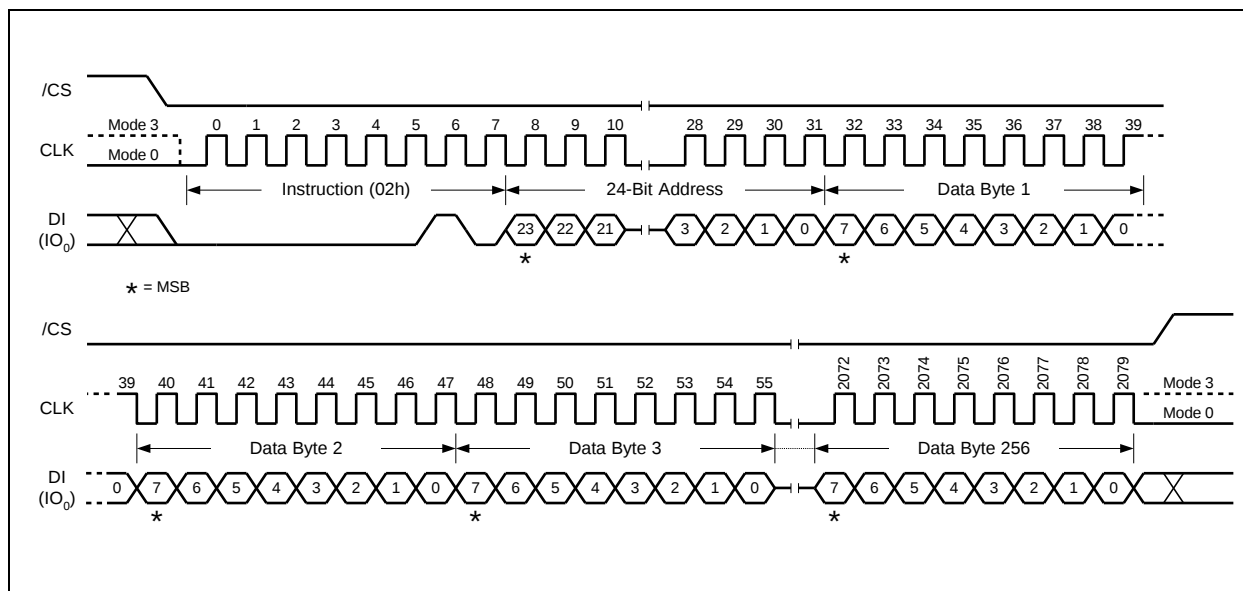
Figure 23a. Page Program Instruction (SPI Mode)
