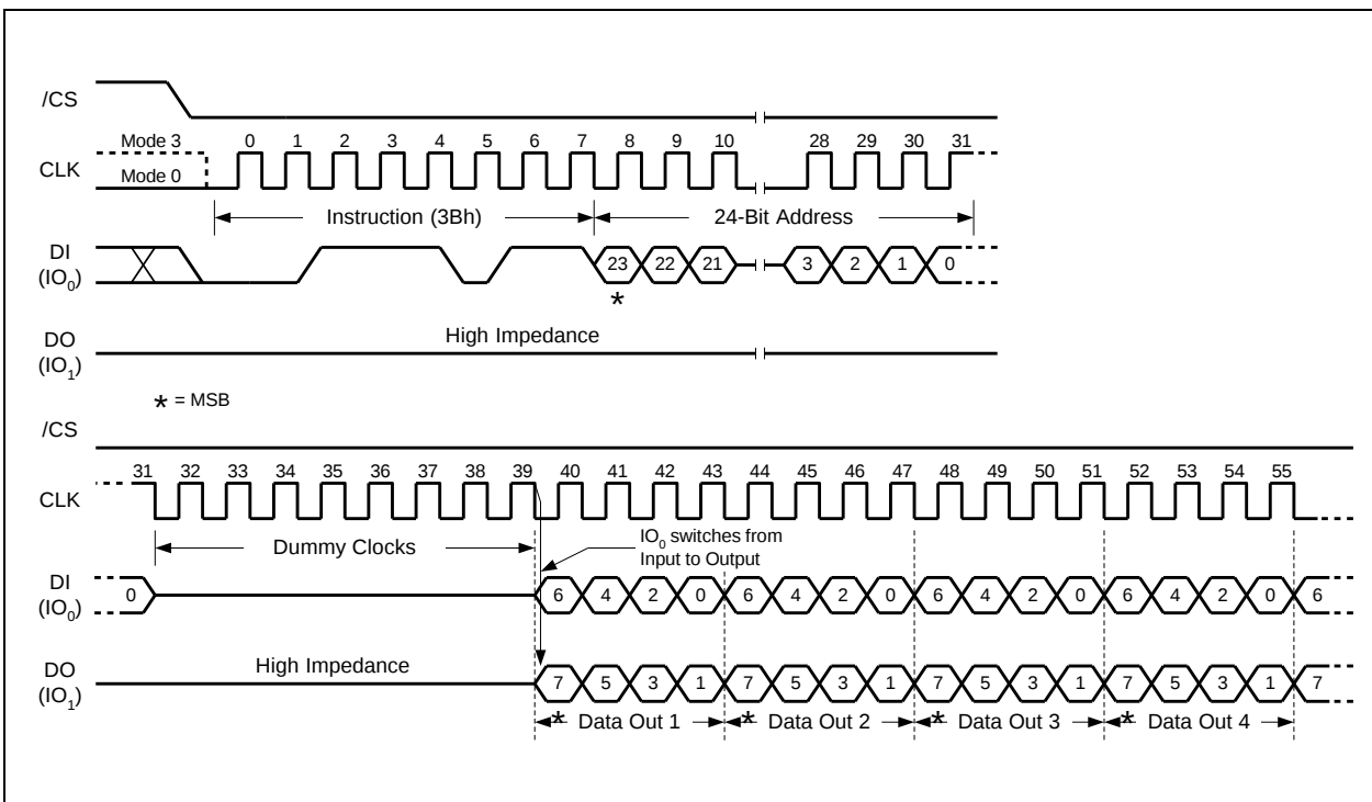
Figure 15. Fast Read Dual Output Instruction (SPI Mode only)
