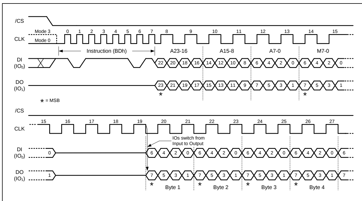
Figure 18a. DTR Fast Read Dual I/O (Initial instruction or previous M5-4≠10, SPI Mode only)
