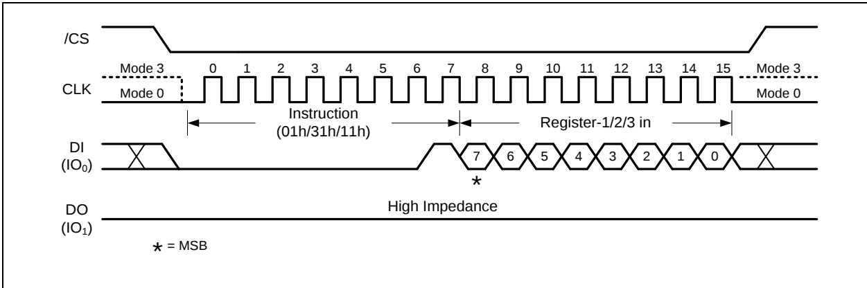
Figure 10a. Write Status Register-1/2/3 Instruction (SPI Mode)
