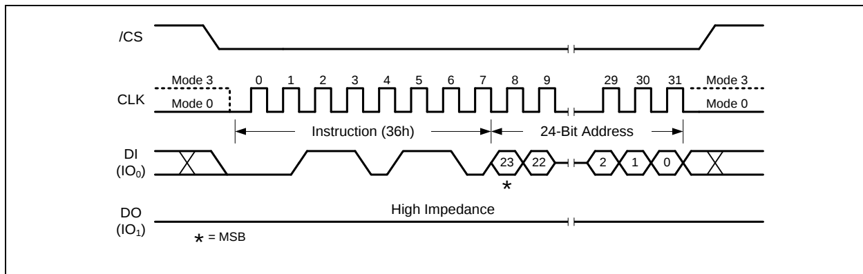
Figure 47a. Individual Block/Sector Lock Instruction (SPI Mode)
