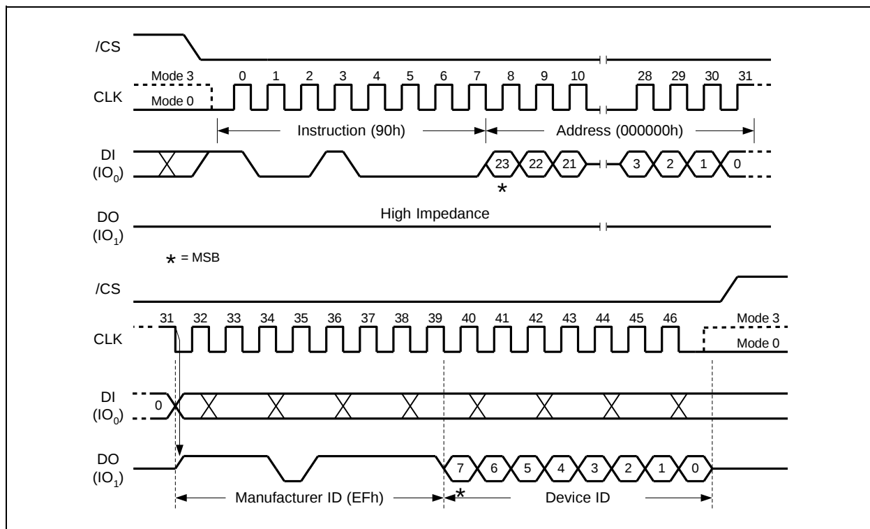
Figure 33. Read Manufacturer / Device ID Instruction (SPI Mode)
