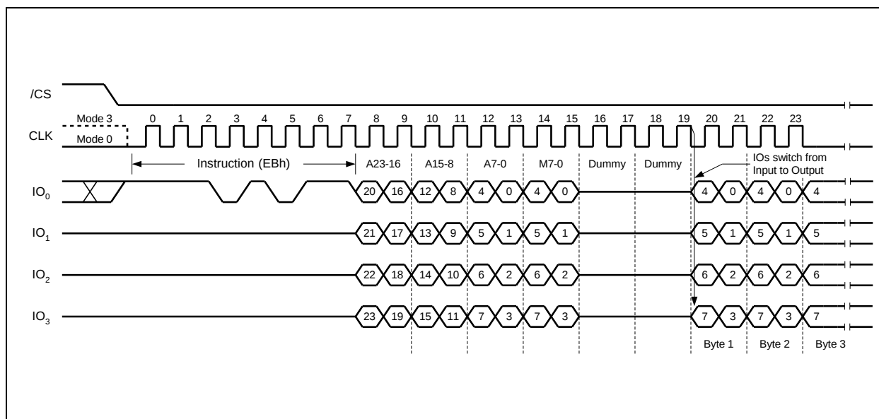
Figure 19a. Fast Read Quad I/O Instruction (Initial instruction or previous M5-4≠10, SPI Mode)
