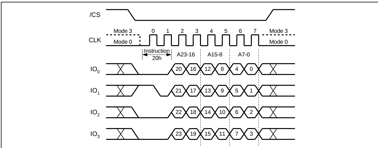
Figure 25b. Sector Erase Instruction (QPI Mode)
