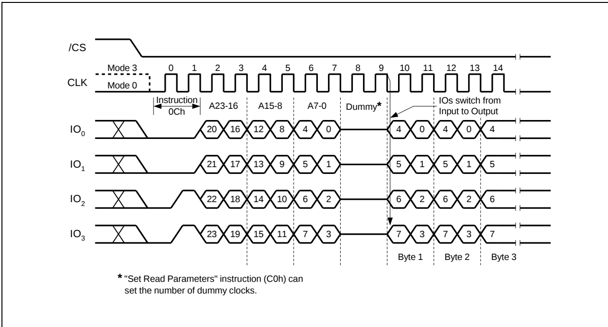
Figure 43. Burst Read with Wrap Instruction (QPI Mode only)
