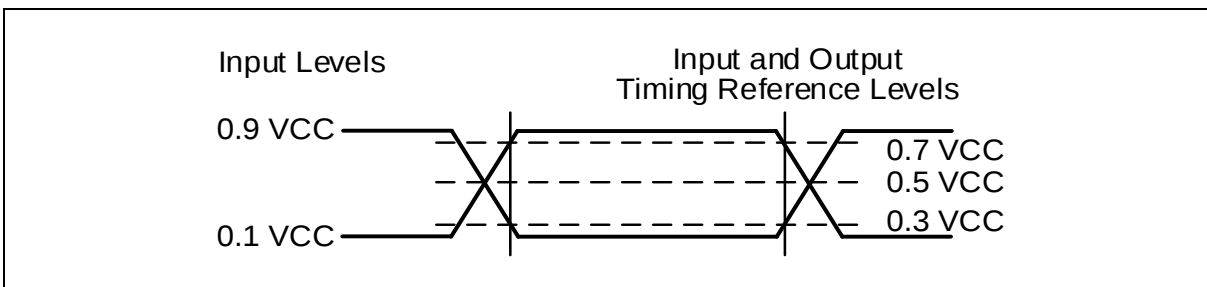
Figure 54. AC Measurement I/O Waveform
