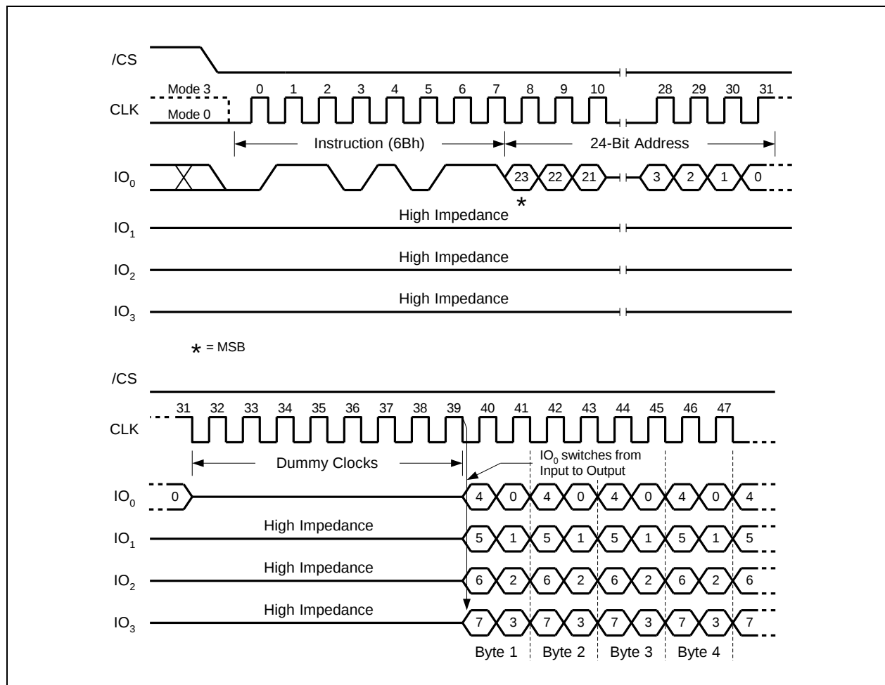
Figure 16. Fast Read Quad Output Instruction (SPI Mode only)
