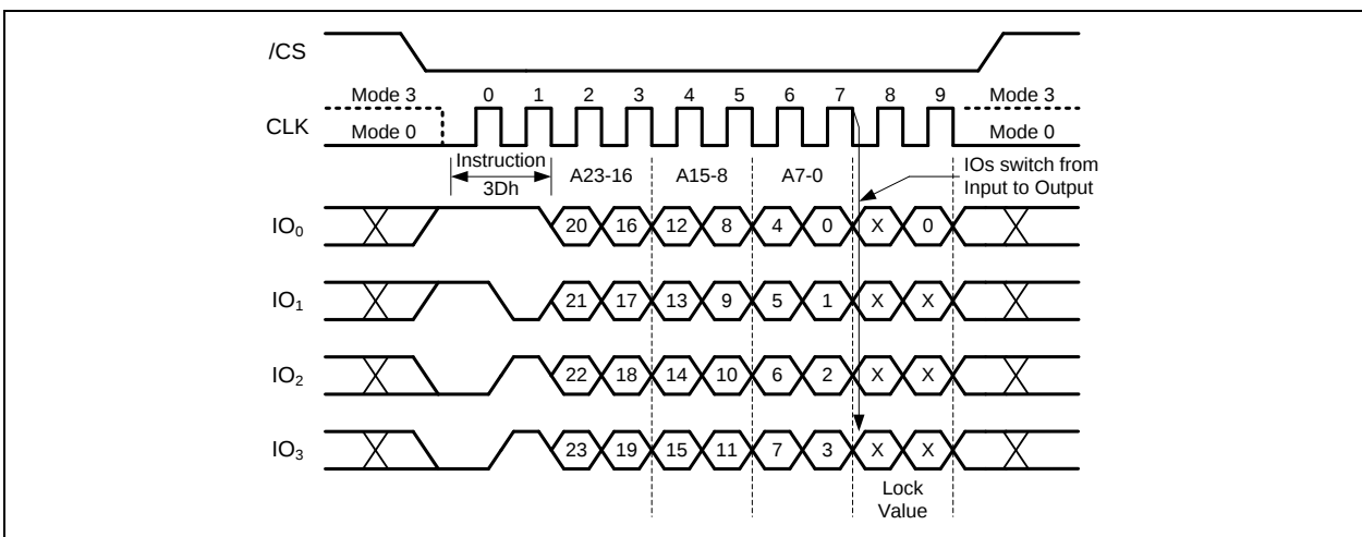
Figure 49b. Read Block Lock Instruction (QPI Mode)
