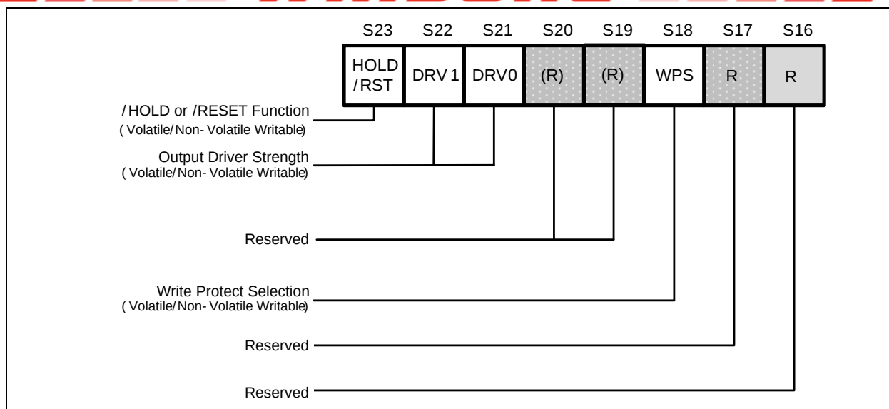
Figure 4c. Status Register-3
