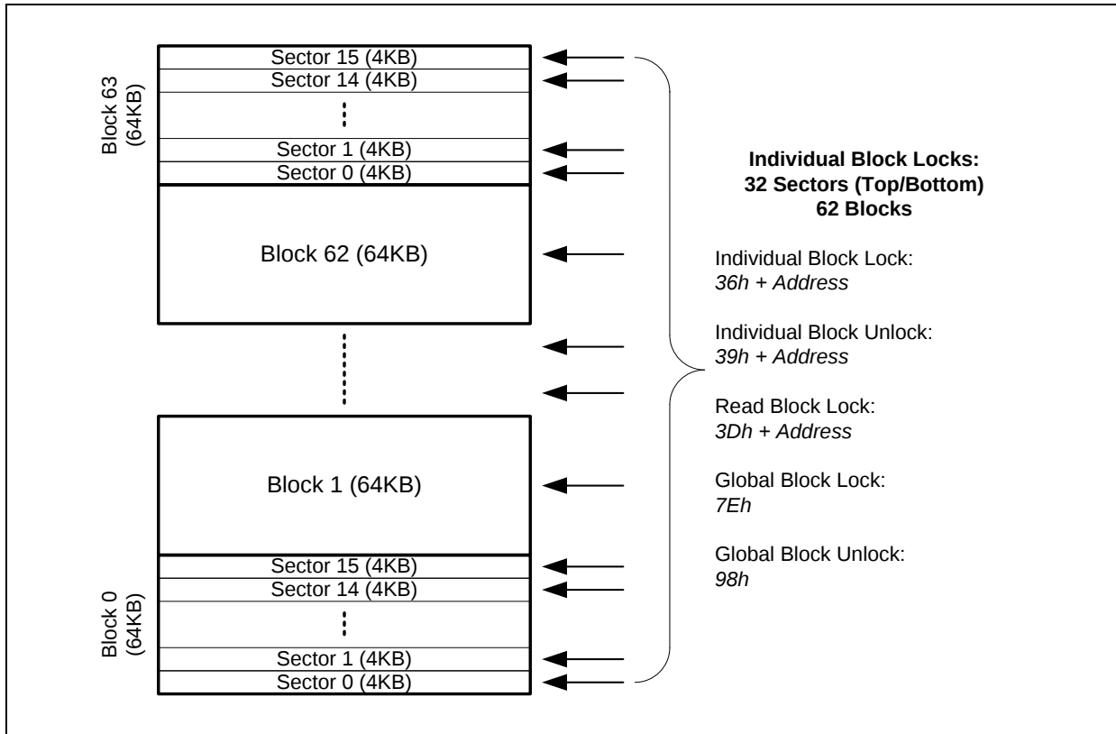
Figure 5. Individual Block/Sector Locks
