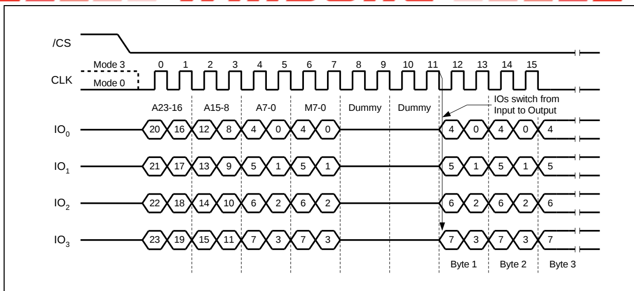
Figure 19b. Fast Read Quad I/O Instruction (Previous instruction set M5-4 = 10, SPI Mode)
