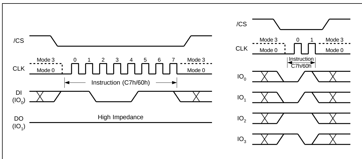
Figure 28. Chip Erase Instruction for SPI Mode (left) or QPI Mode (right)
