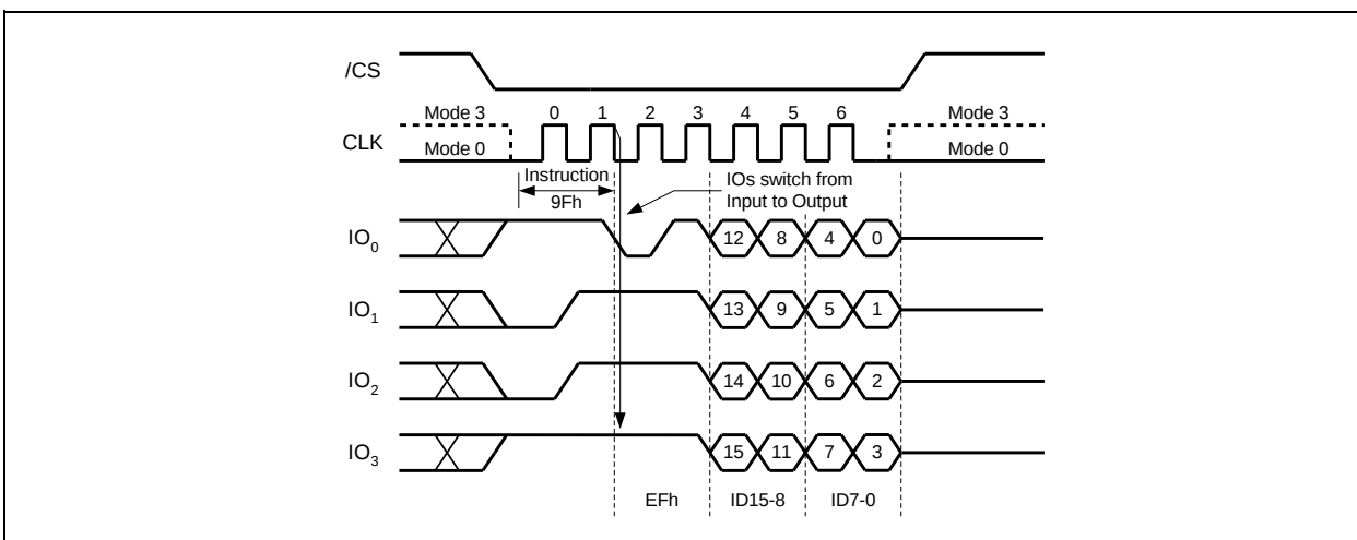
Figure 37b. Read JEDEC ID Instruction (QPI Mode)
