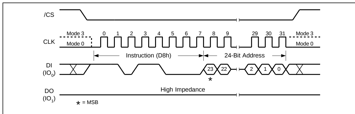
Figure 27a. 64KB Block Erase Instruction (SPI Mode)
