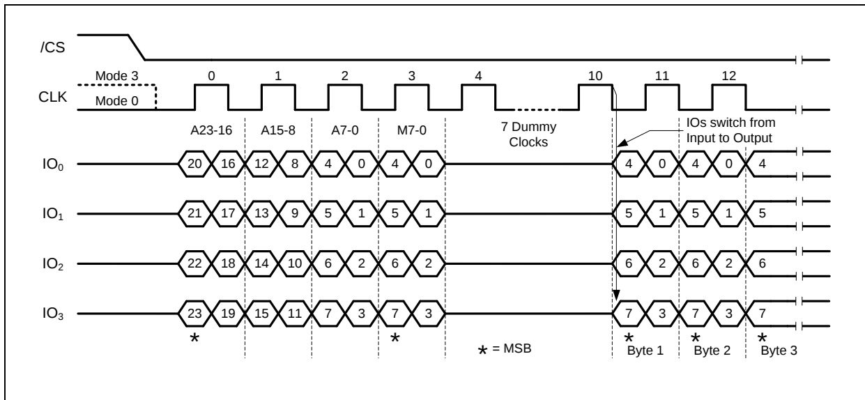
Figure 20b. Fast Read Quad I/O (Previous instruction set M5-4=10, SPI Mode)
