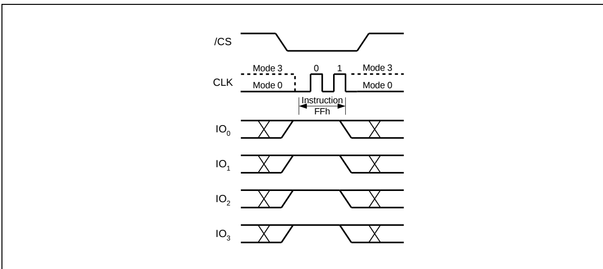
Figure 46. Exit QPI Instruction (QPI Mode only)
