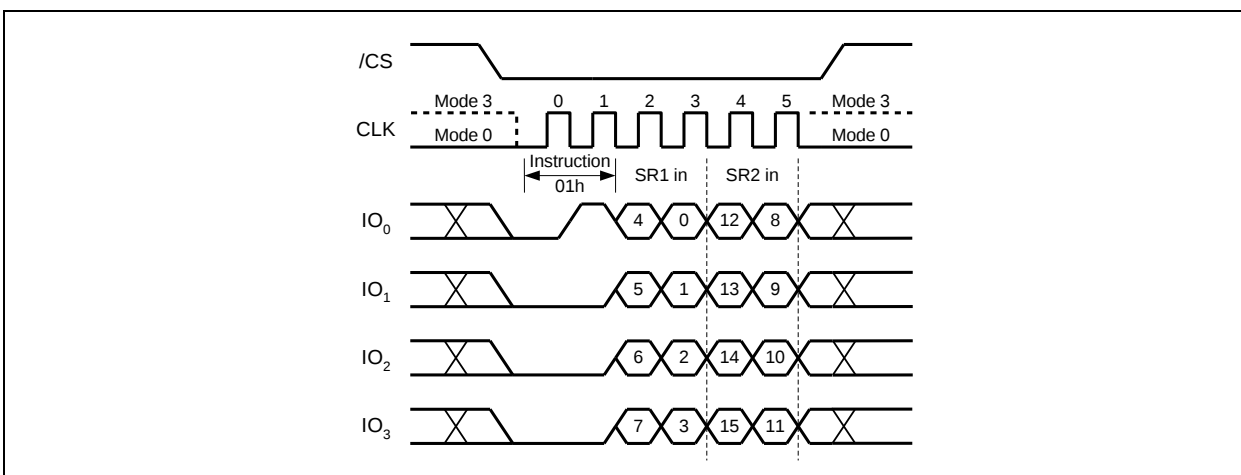
Figure 11b. Write Status Register-1/2 Instruction (QPI Mode)
