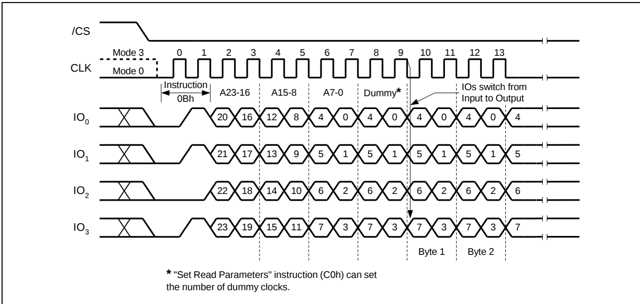
Figure 13b. Fast Read Instruction (QPI Mode)
