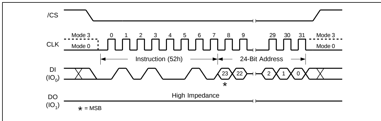
Figure 26a. 32KB Block Erase Instruction (SPI Mode)
