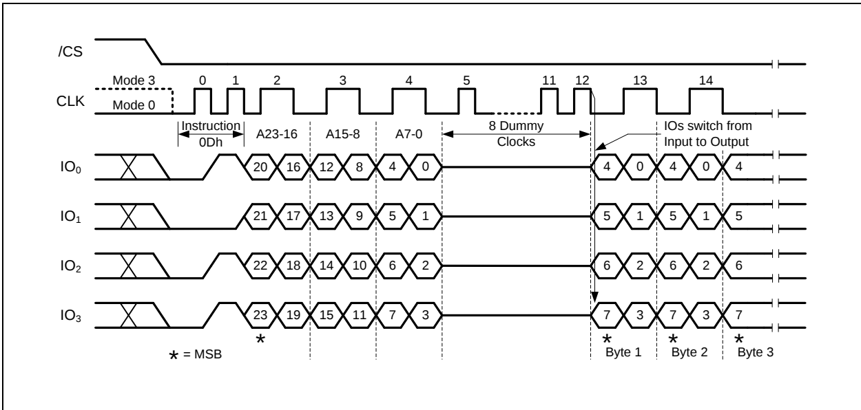
Figure 14b. DTR Fast Read Instruction (QPI Mode)
