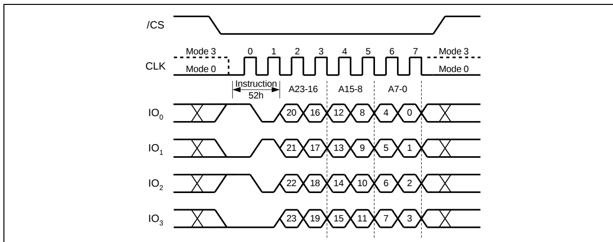
Figure 26b. 32KB Block Erase Instruction (QPI Mode)
