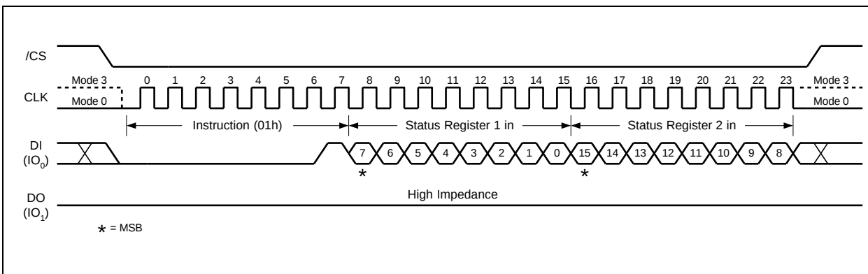
Figure 11a. Write Status Register-1/2 Instruction (SPI Mode)
