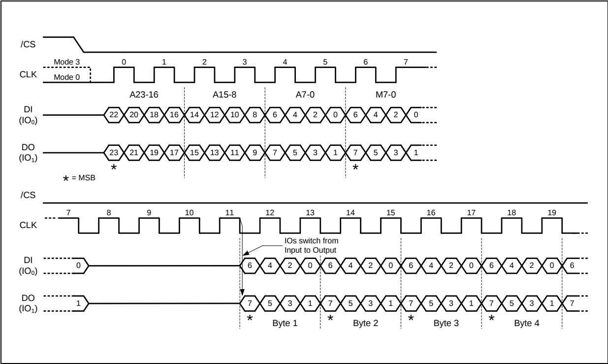
Figure 18b. DTR Fast Read Dual I/O (Previous instruction set M5-4=10, SPI Mode only)
