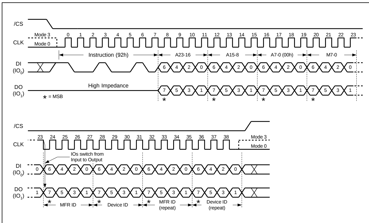
Figure 34. Read Manufacturer / Device ID Dual I/O Instruction (SPI Mode only)
