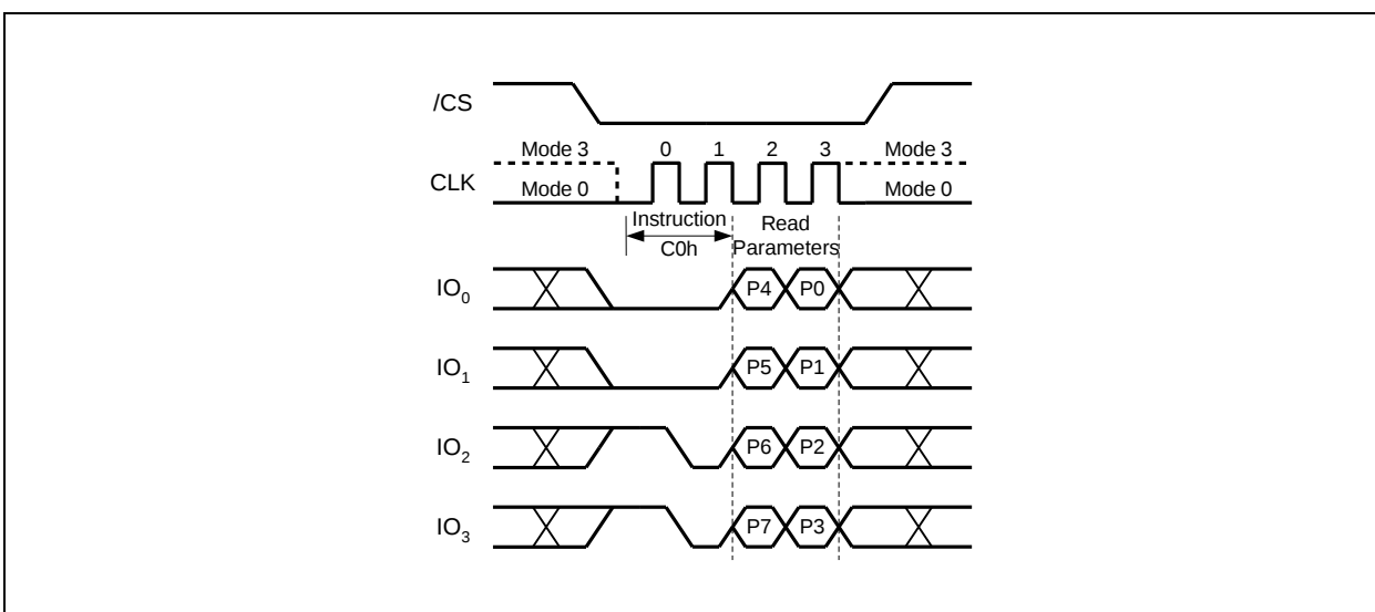
Figure 42. Set Read Parameters Instruction (QPI Mode only)
