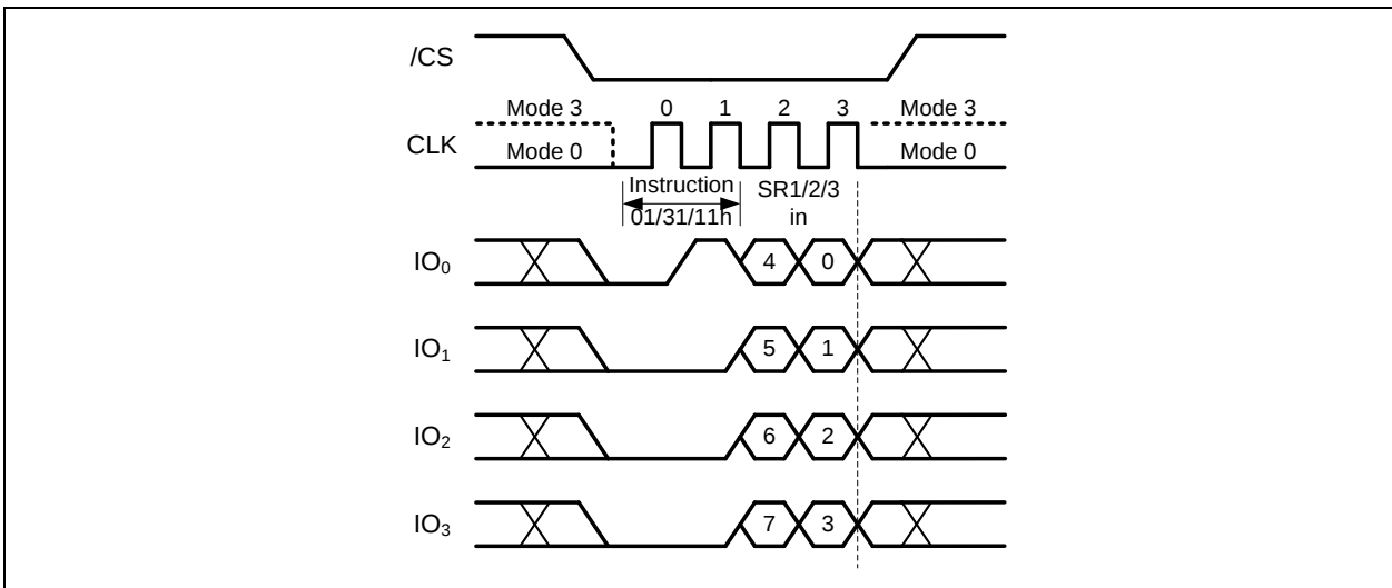
Figure 10b. Write Status Register-1/2/3 Instruction (QPI Mode)
