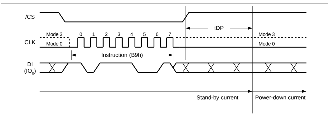
Figure 31a. Deep Power-down Instruction (SPI Mode)
