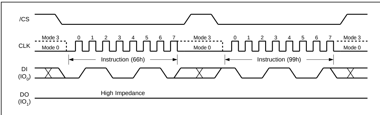
Figure 52a. Enable Reset and Reset Instruction Sequence (SPI Mode)
