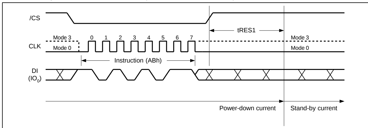
Figure 32a. Release Power-down Instruction (SPI Mode)
