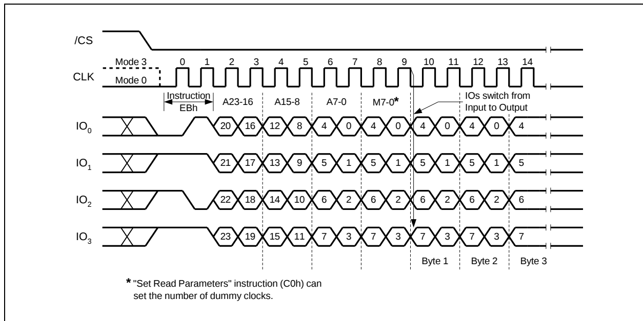
Figure 21b. Fast Read Quad I/O Instruction (Initial instruction or previous M5-4≠10, QPI Mode)
