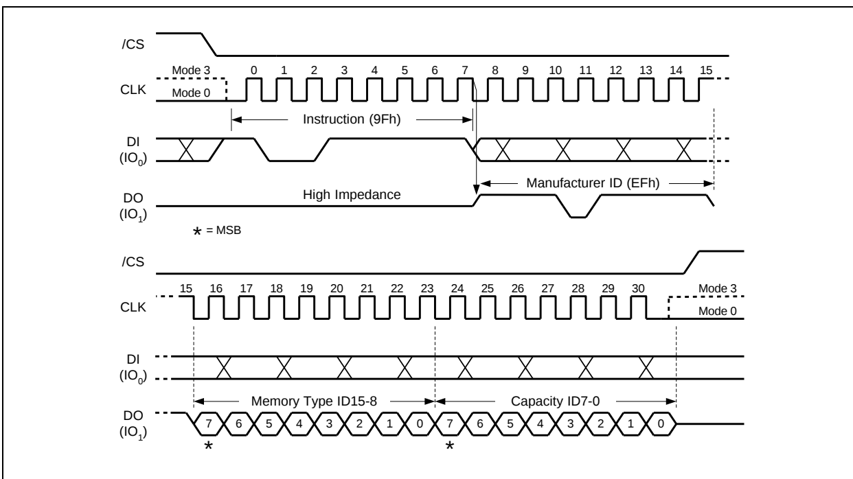
Figure 37a. Read JEDEC ID Instruction (SPI Mode)
