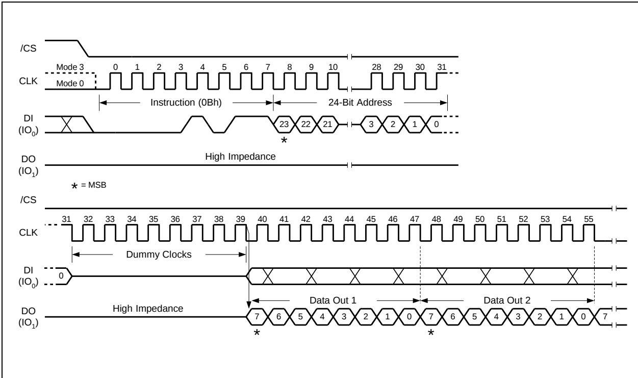
Figure 13a. Fast Read Instruction (SPI Mode)
