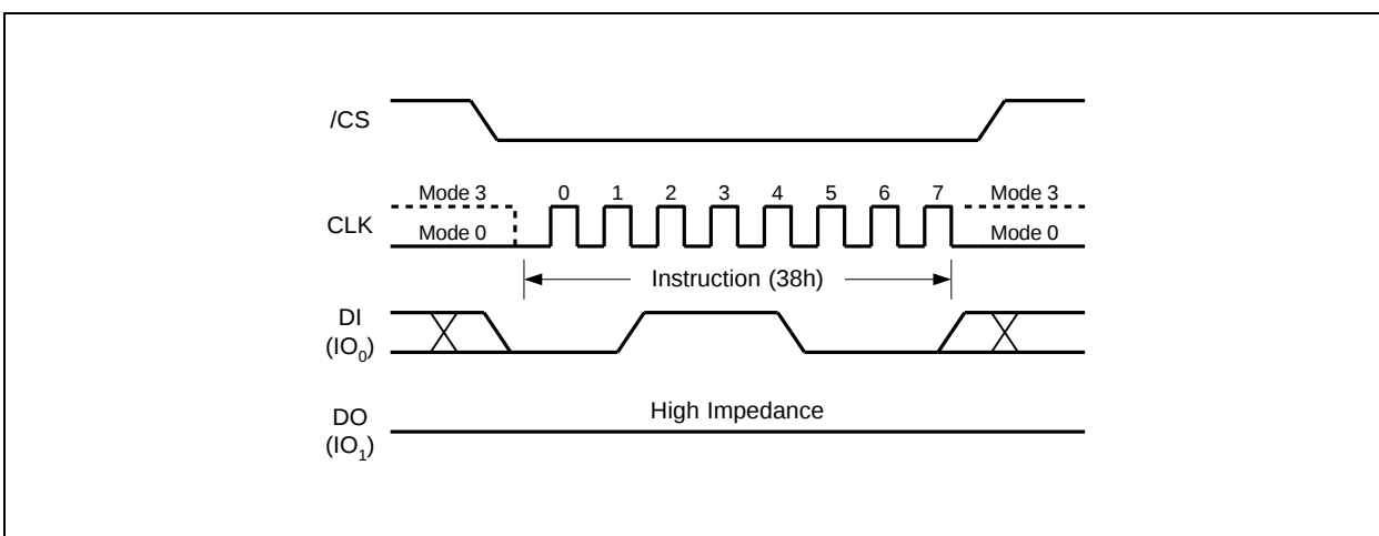
Figure 45. Enter QPI Instruction (SPI Mode only)
