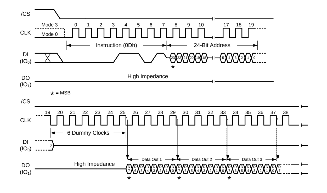
Figure 14a. DTR Fast Read Instruction (SPI Mode)
