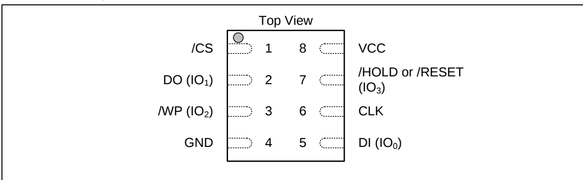
Figure 1b. W25Q32JV Pad Assignments, 8-pad W/X/USON 6x5/4x4/4x3-mm (Package Code ZP/XG/UU)
