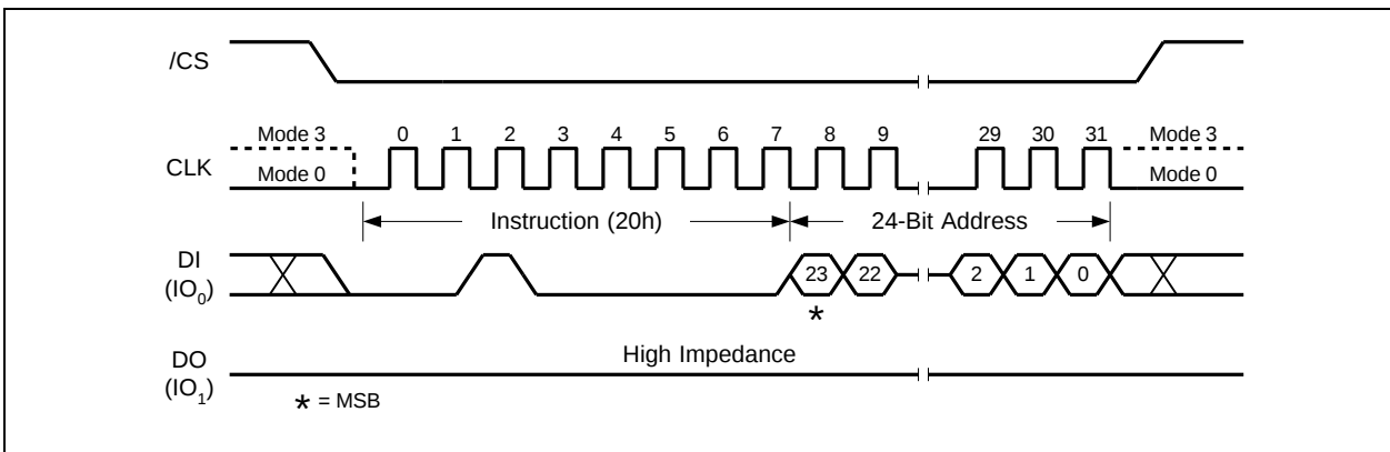
Figure 25a. Sector Erase Instruction (SPI Mode)
